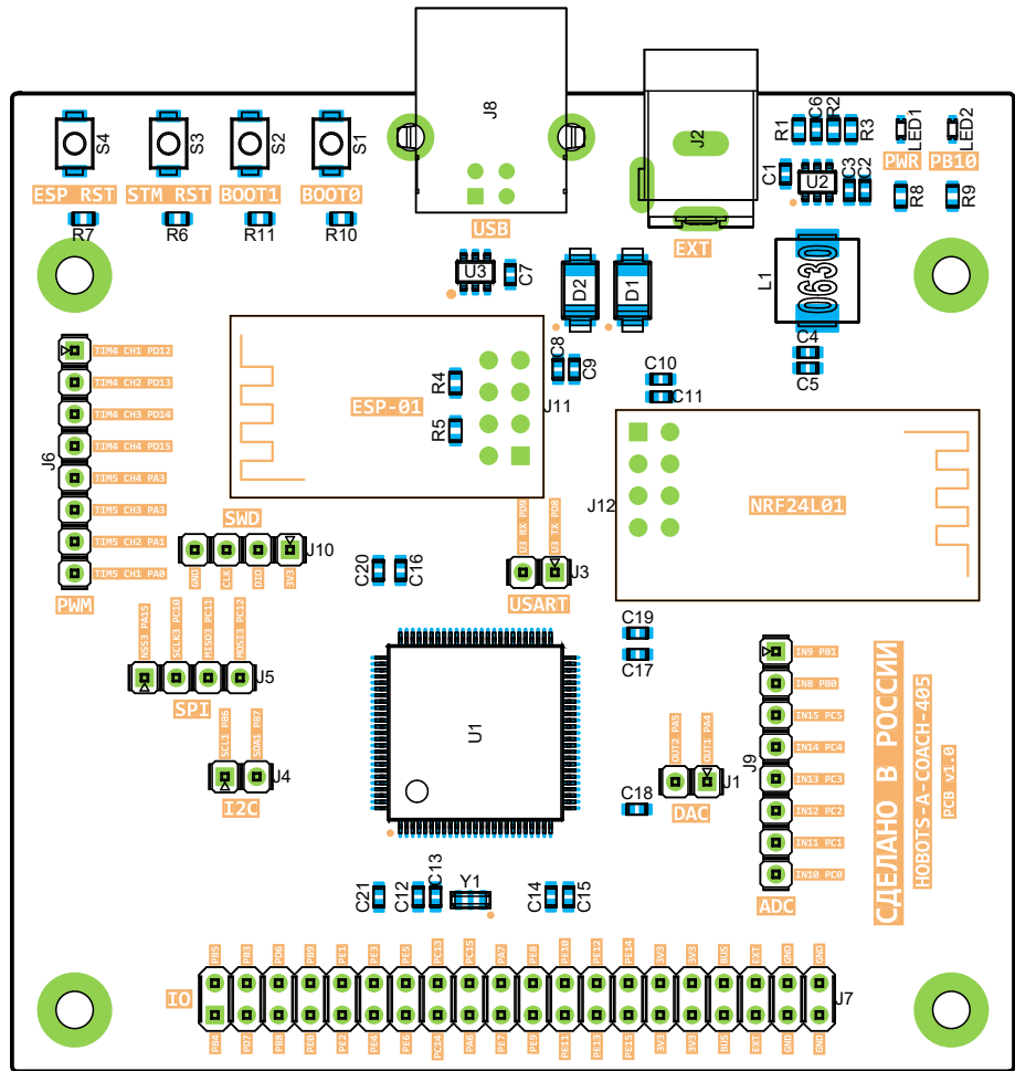
View from Top side (Scale 3:2)
